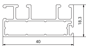
VR032 Traverse 12 mm
