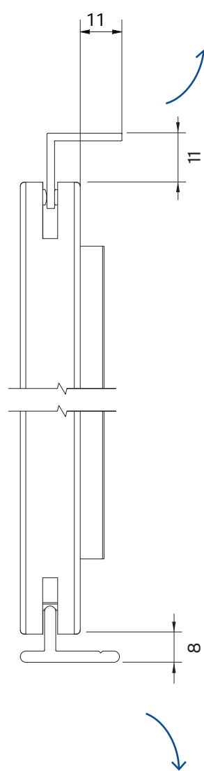
VP1016 Rail plat 15 mm
