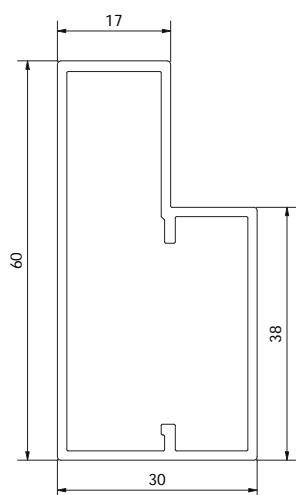
VP1005 Traverse
